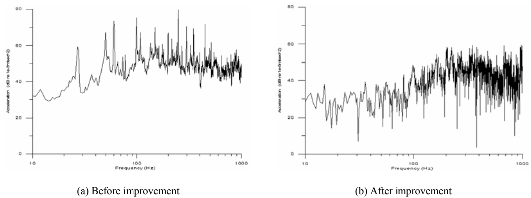
Fig. 17. Transmitted vibration acceleration spectrum at B during operation of parking tower.
