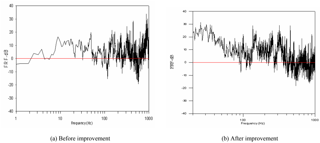
Fig. 15. Vibration isolation via mount D.
