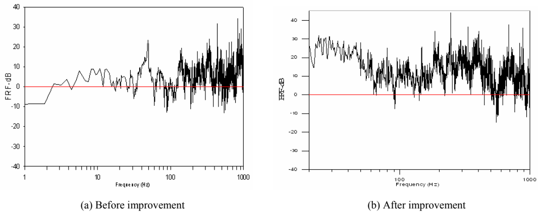
Fig. 16. Vibration isolation via mount F.
