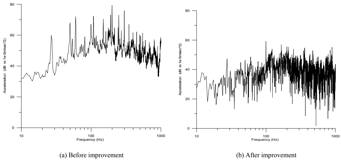
Fig. 18. Transmitted vibration acceleration spectrum at E during operation of parking tower.
